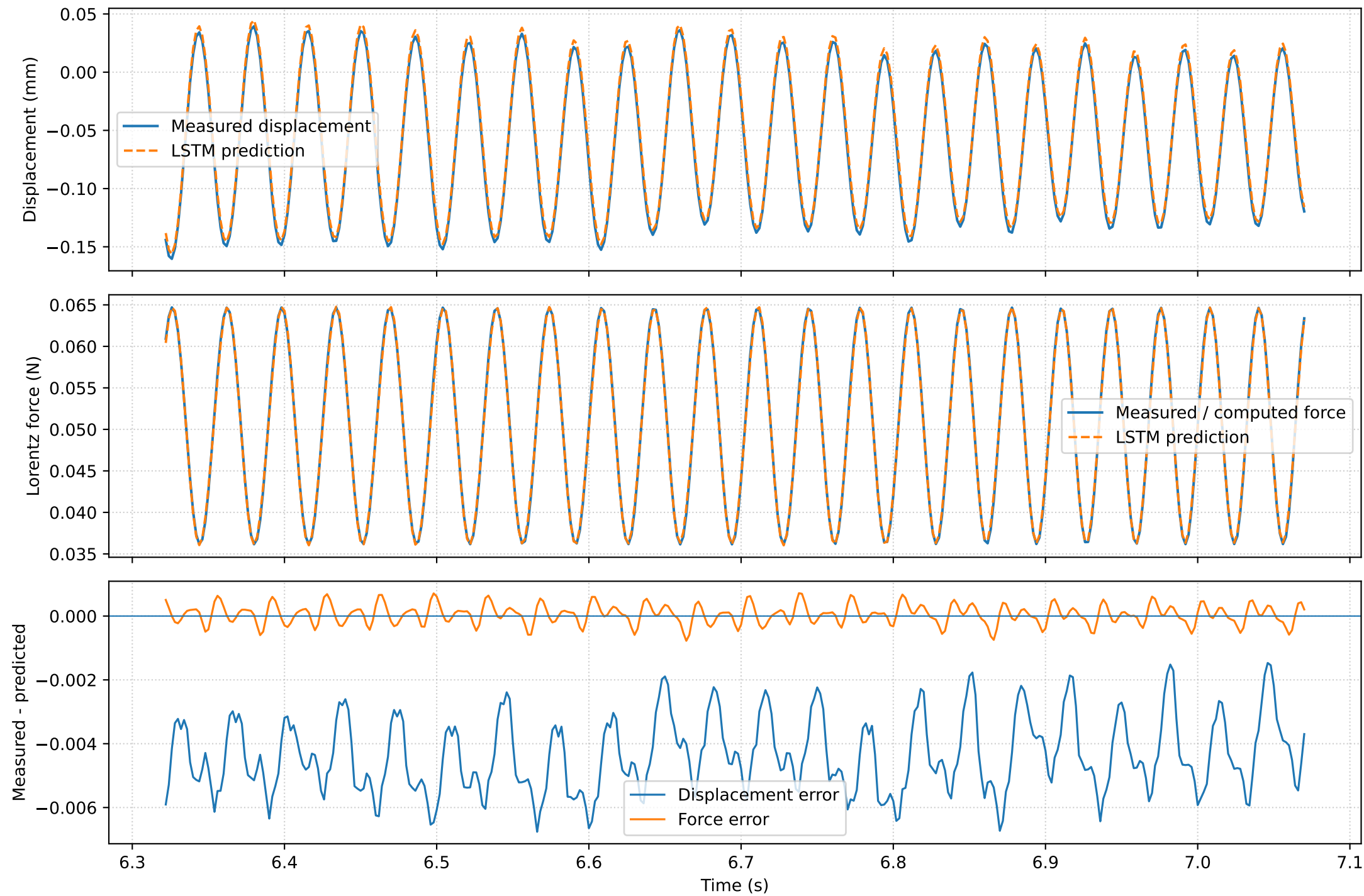
Zoomed LSTM tracking: Chirp_2 | center = 6.696 s | window = 0.750 s
